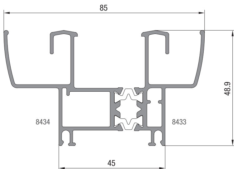
RPT-030 1.513 kg/m
